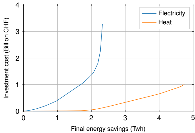
Figure 6: Energy efficiency cost curve for the Swiss industry.
